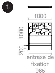
Fixing principle
