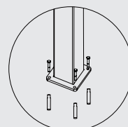
Fixing principle
