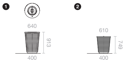
Bottom view (with fixing centers)
