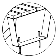
Fixing principle
