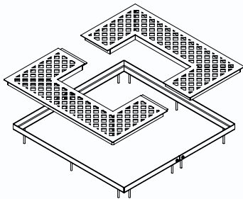
Fixing principle, by sealant
